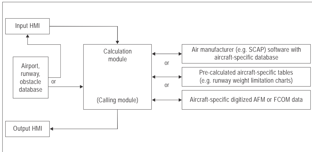
Figure A-1. Typical architecture of a performance application
